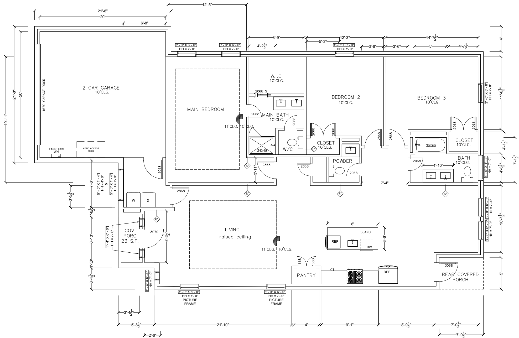
Floor Plan - Proposed
