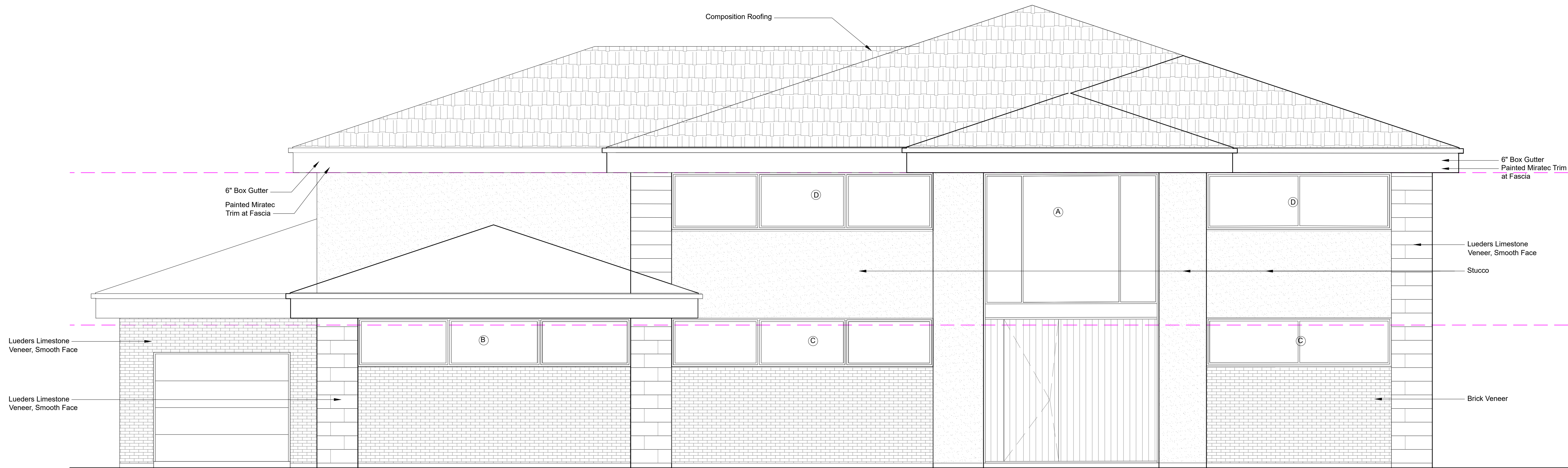
1. EXTERIOR ELEVATION: front, southeast
