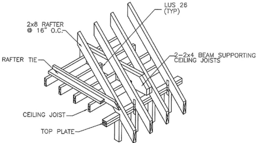
TYPICAL BEAM & RAFTER TIE DETAIL not to scale
