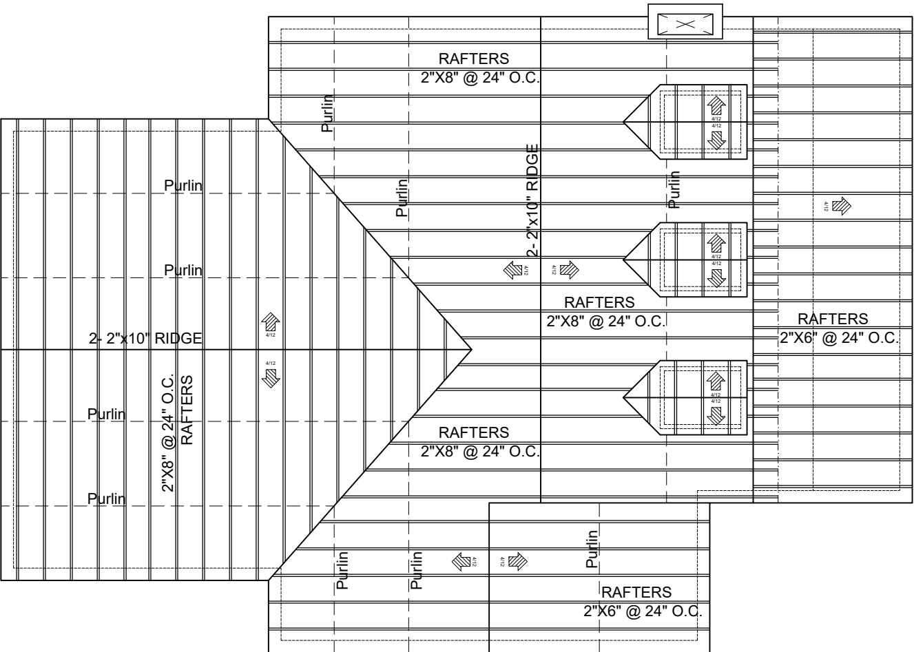
ROOF PLAN SCALE 3/32" = 1'-0"
